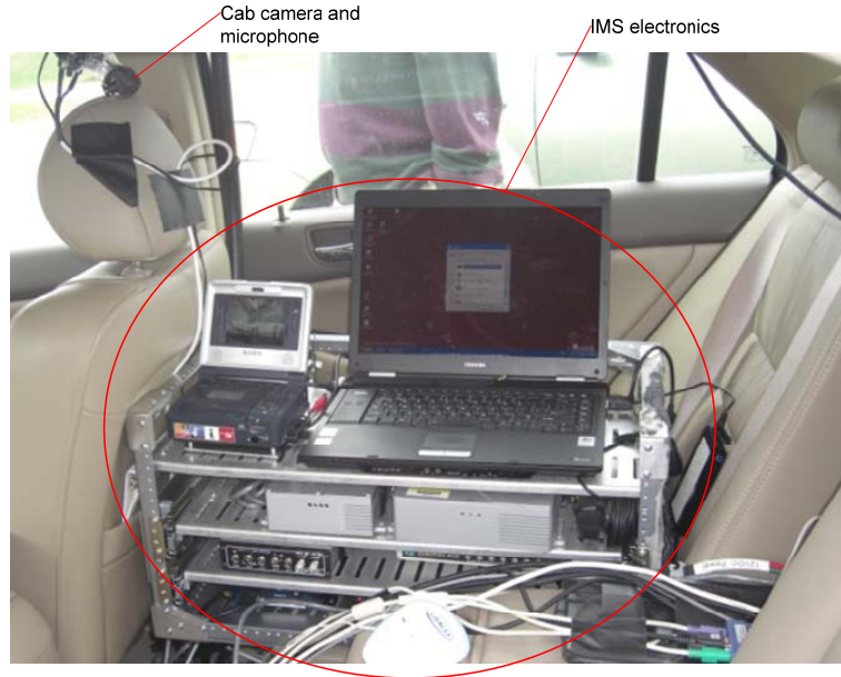
Figure 5. Measurement system electronics in back seat of light vehicle.
